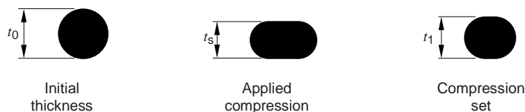
Figure 6 – Compression set of an O-ring
