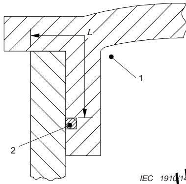
Figure 10 – Illustration of the requirements concerning gaskets – Example 1
