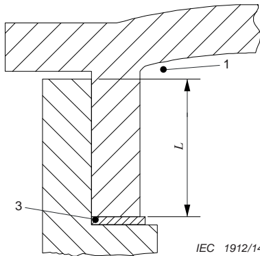
Figure 12 – Illustration of the requirements concerning gaskets – Example 3
