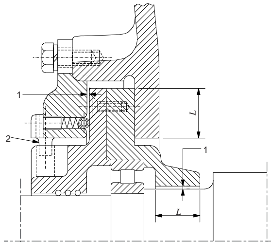
Figure 18 – Example of labyrinth joint for shaft of rotating electrical machine
