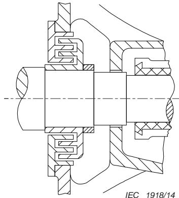
Figure 17 – Example of cylindrical joint for shaft of rotating electrical machine
